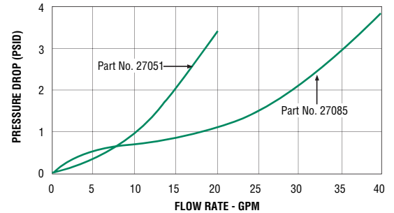
2" NPT Ports
