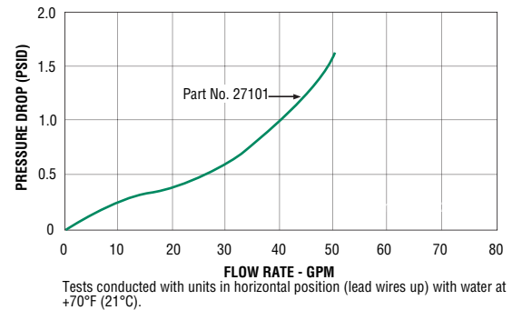
2" NPT Ports
