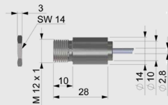
Sensing head
