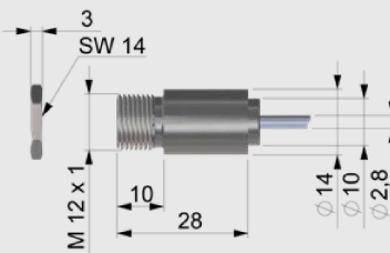
Sensing head
