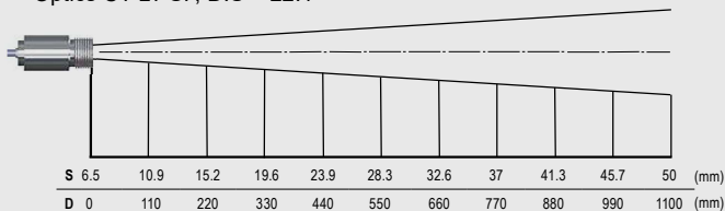
Optics CT LT SF, D:S = 22:1
