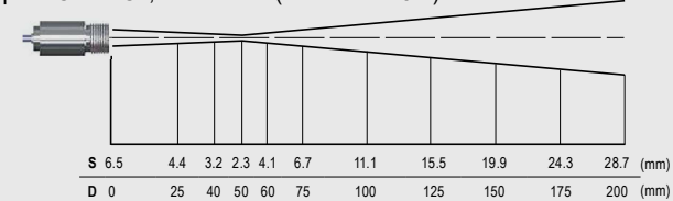
Optics CT LT CF, D:S = 22:1 (far field = 1.5:1)
