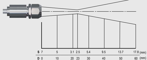
Optics CT LT CF, D:S = 2:1 (far field = 2.5:1)
