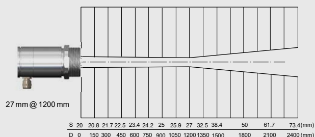
Chart SF optics, D:S = 45:1
